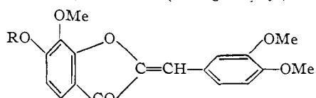
VI, heptamethylmaritimoin (R = tetramethylglucosidyl)
