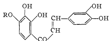
I, marein (R = glucosidyl) II, okanin (R = H)
