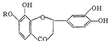
III, flavanomarein (R = glucosidyl) IV, probably isoökanin (R = H)
