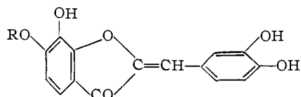
V, maritimoin (R = glucosidyl)
