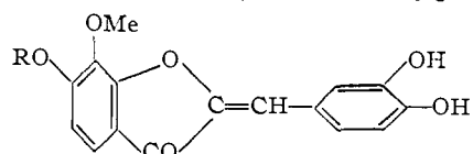
VII, leptosin (R = glucosidyl) VIII, leptosidin (R = H)
